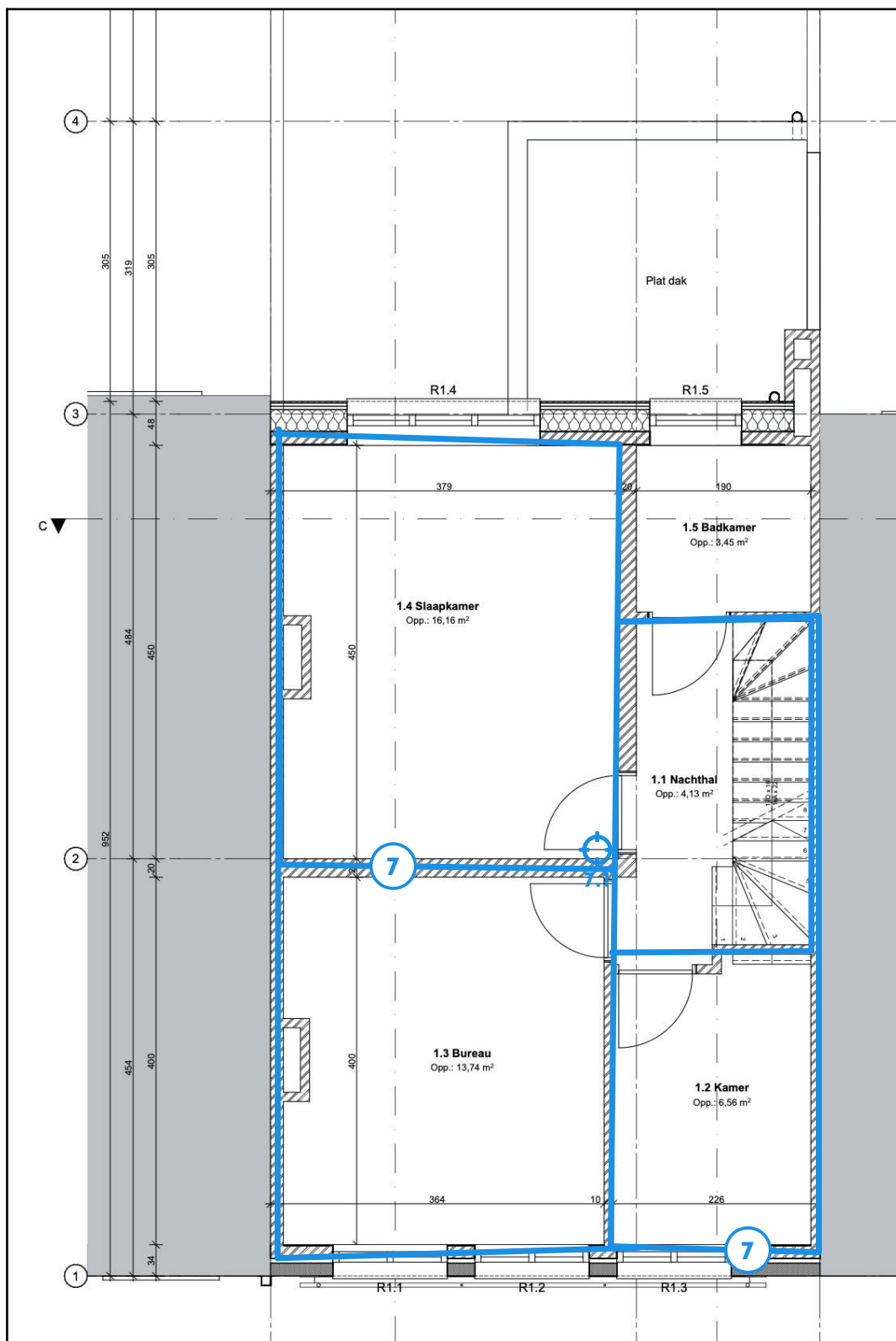
Legende van plan 1.6: Plan woning +1
