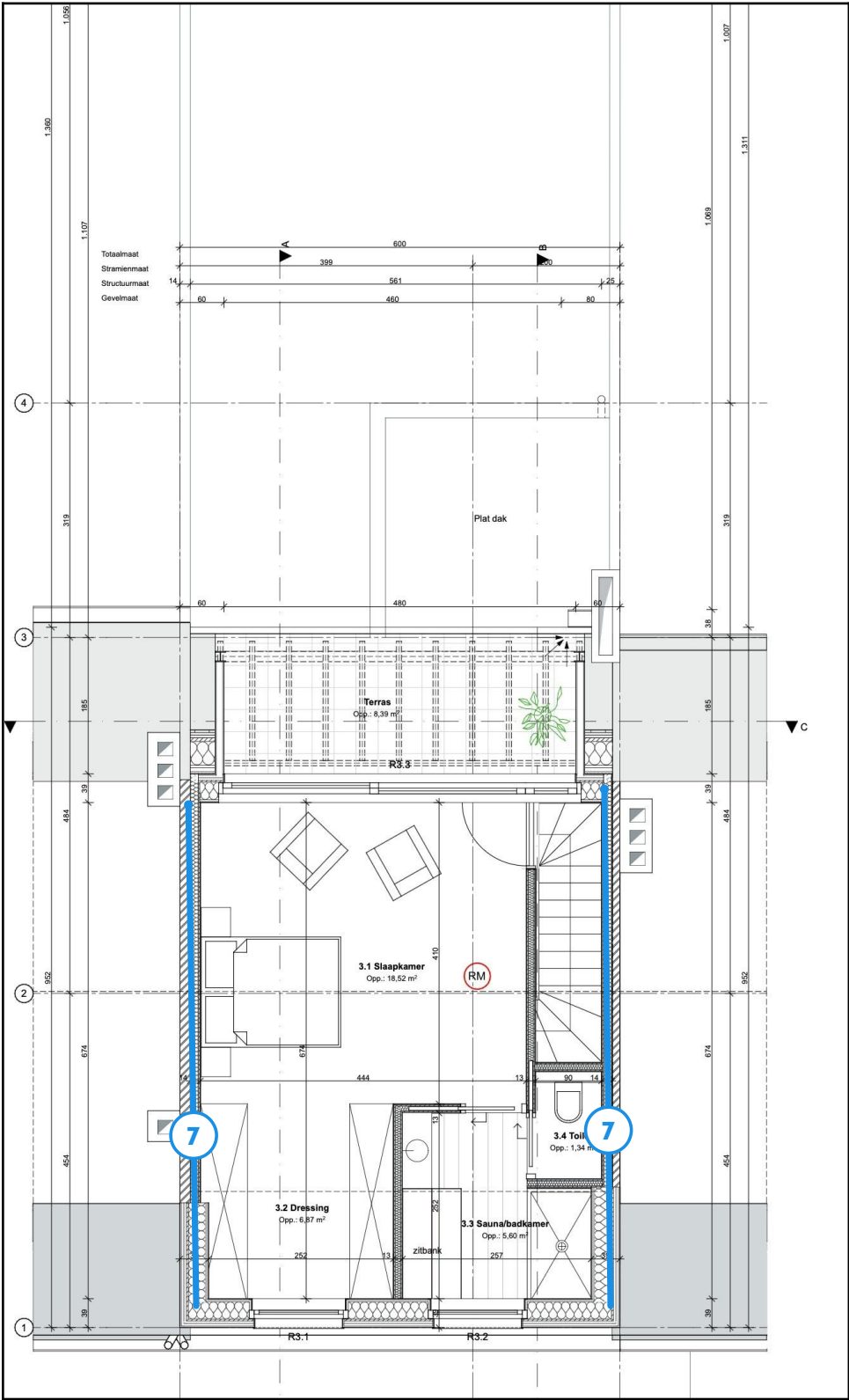
Legende van plan 1.13: Plan woning +3
