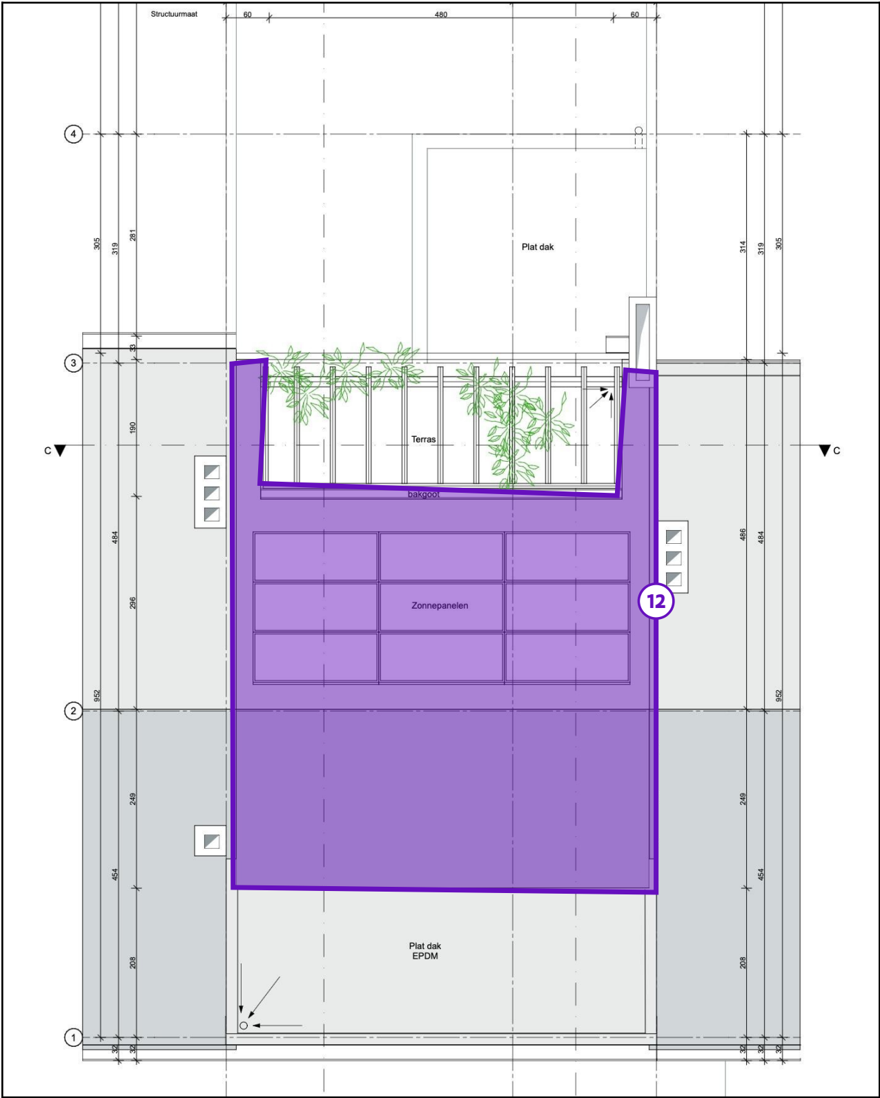
Legende van plan 1.16: Plan dak
